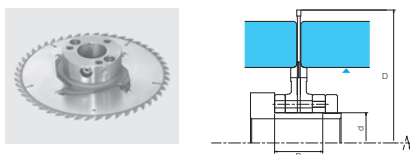
3 rd horizontal profiling bottom side and splitting
