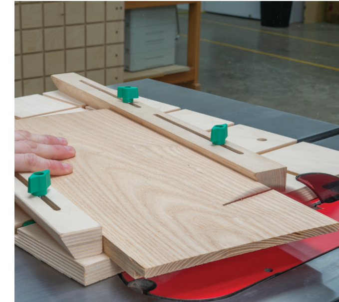
No matter the angle of your cut the Miter Bars keep the sled moving parallel to the blade at all times.
