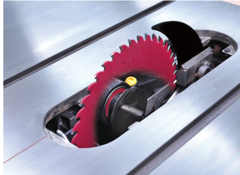
Add multiple Arbor Shims and watch your thin kerf blade magically align to the same cut line as a full kerf blade.
